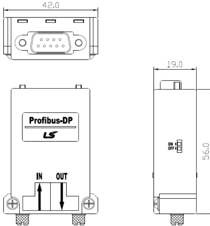
Figure 2 PROFIBUS Connector
