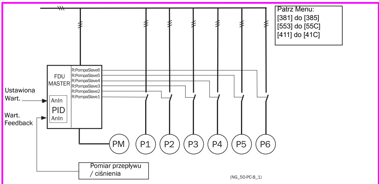
Rys. 72 Regulator PID
