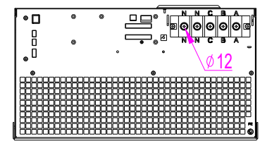
Top View without cable cover
